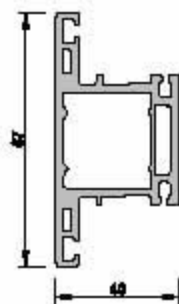
MULLION PROFILE 21601 - 02000 : WHITE
