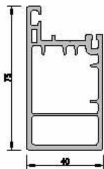
SASH PROFILE 21601 - 01000 : WHITE
