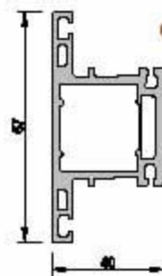
MULLION PROFILE R.21601-02003 : ROBLE
